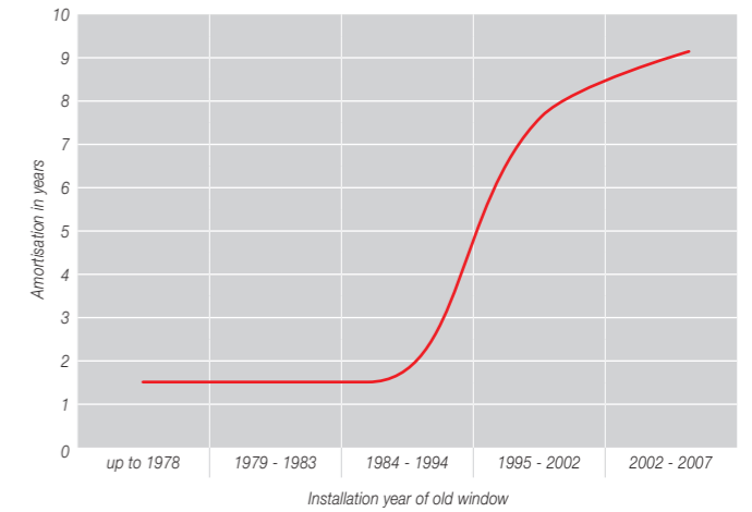
Renovation with WICLINE windows, U_w = 1,0 \text{ W/m}^2\text{K} with thermally insulated triple glazing amortisation when replacing an old aluminium window
